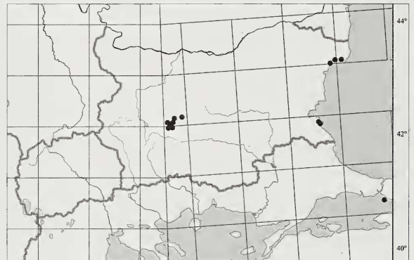
Fig. 1: Localities of Zelotes strandi
